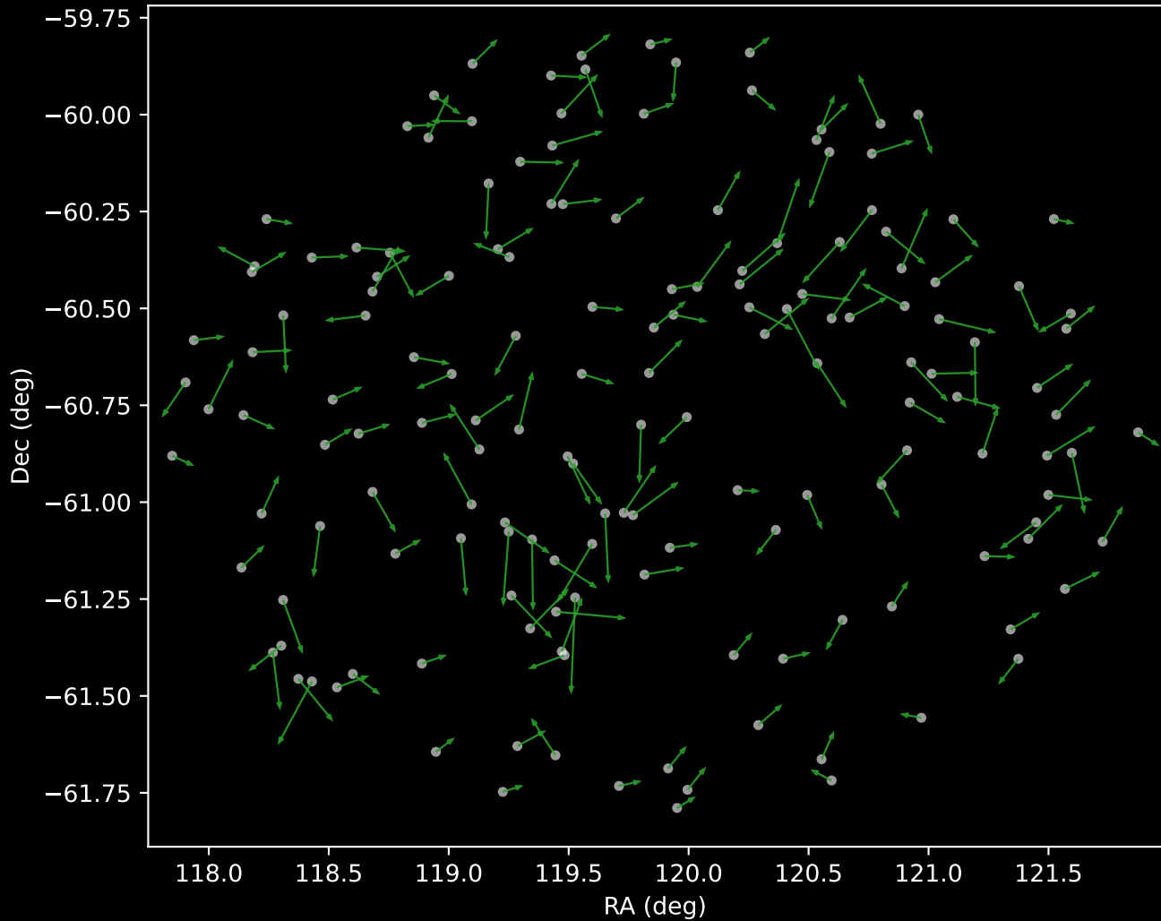
GALAH DR4 Cluster 4 Proper Motion Vectors (n=160)
