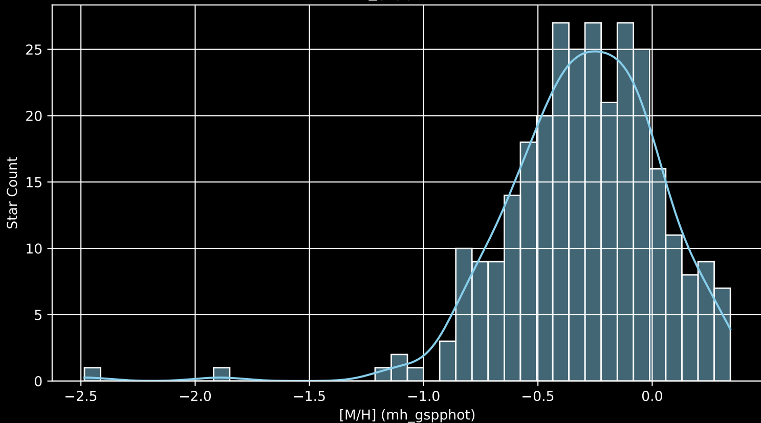
GALAH DR4 Field: [6890] [M/H] (mh_gspphot) (n= 292)
