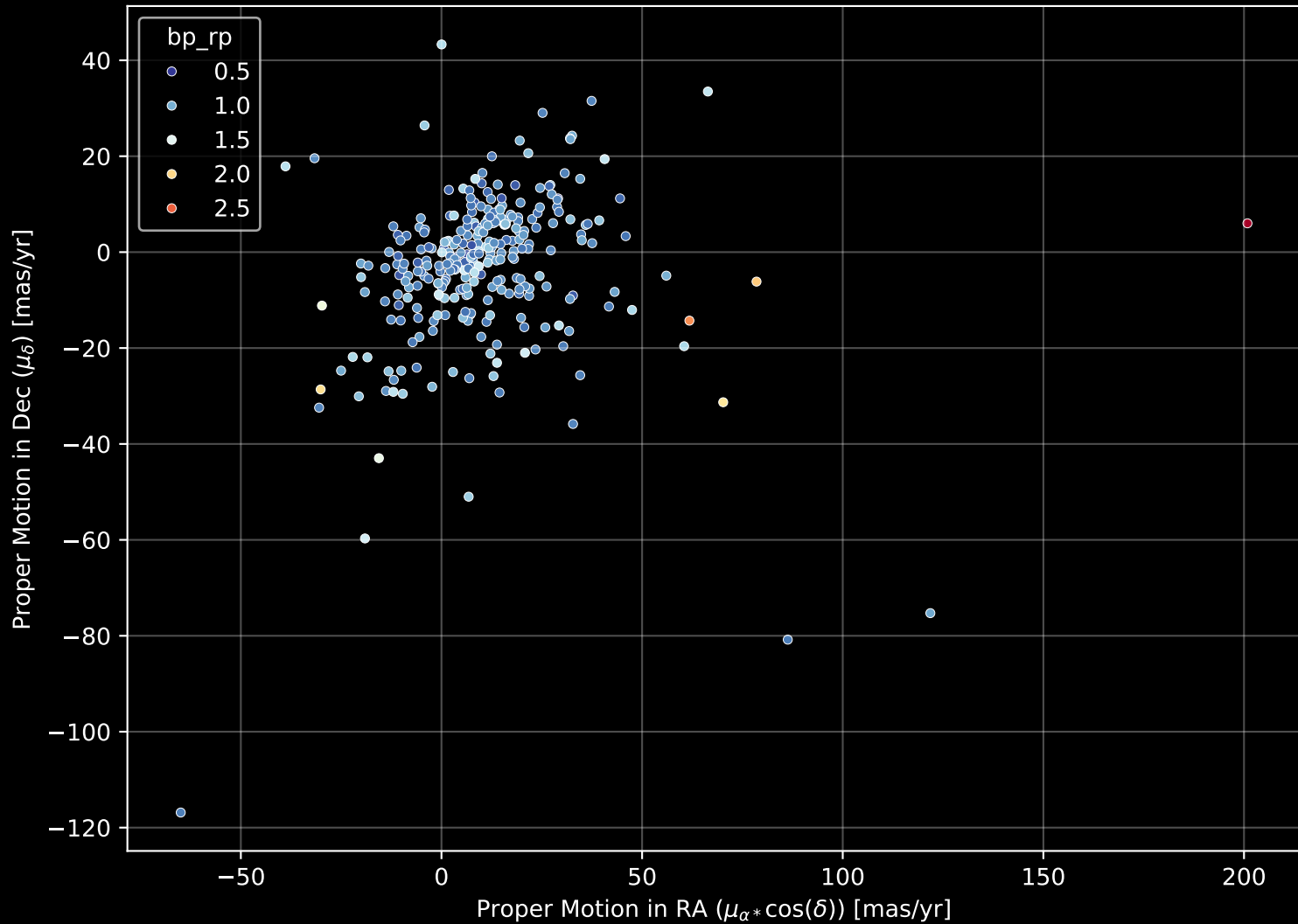
GALAH DR4 Field: [6890] Proper Motion Diagram (n= 293)
