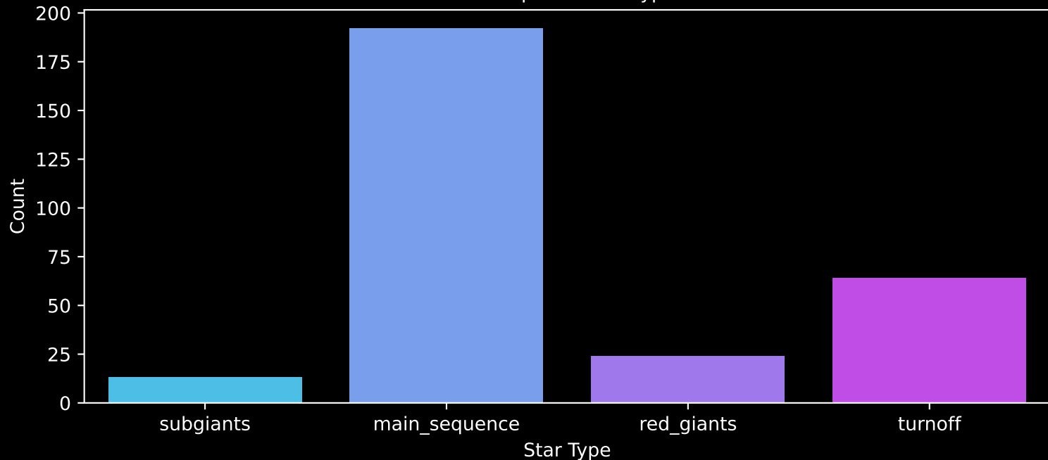
GALAH DR4 Field: [6890] Count plot of Star Type
