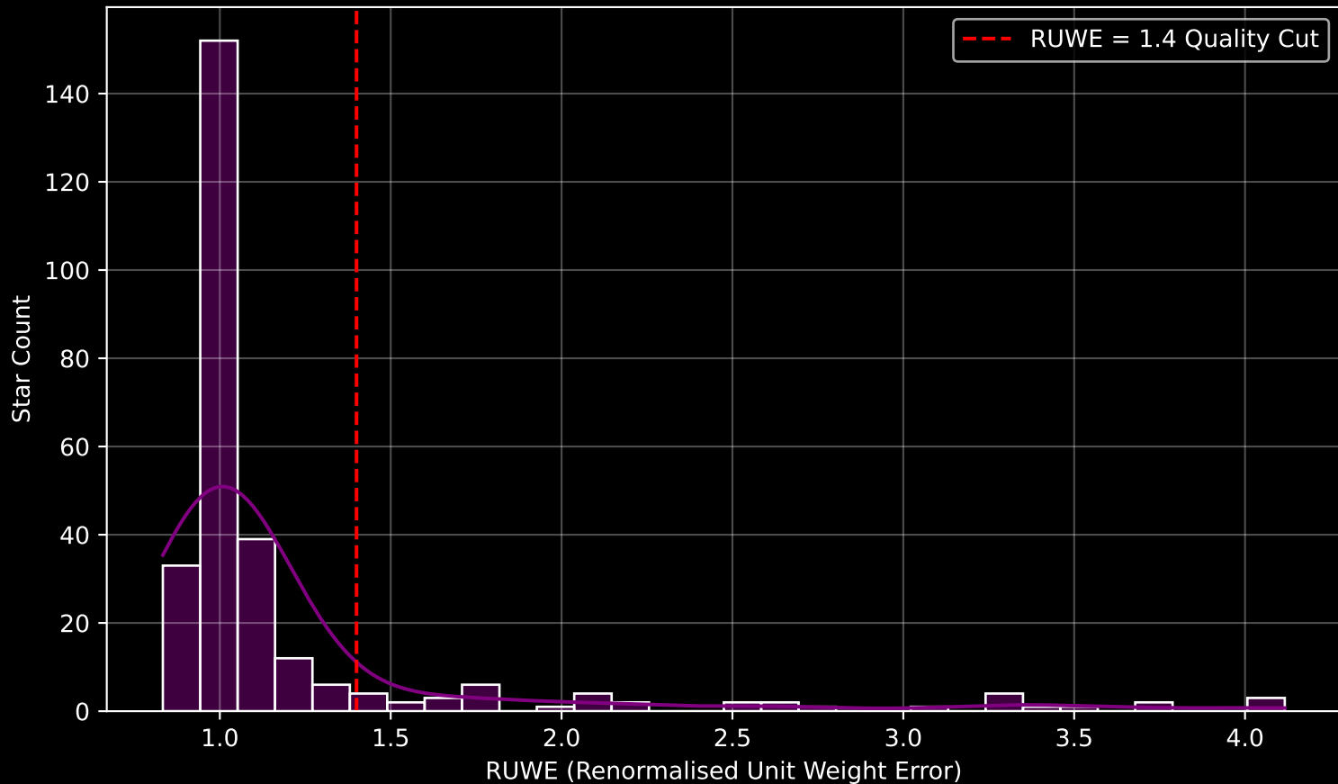
GALAH DR4 Field [6890] RUWE Distribution (n= 281)
