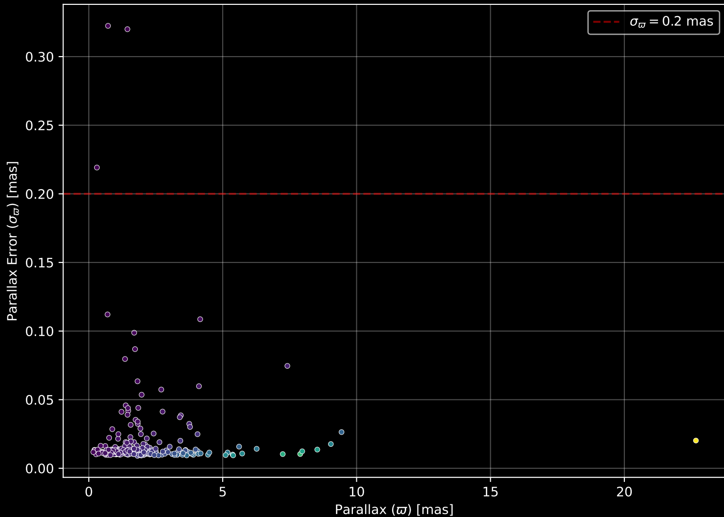
GALAH DR4 Field: [6890] Parallax Quality (n= 293)
